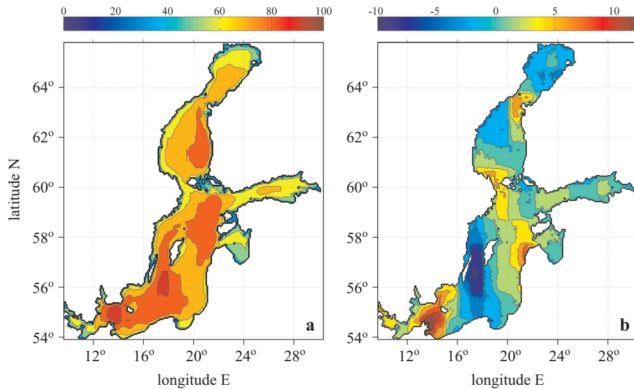
Figure 8. (left) Numerically simulated average significant wave height (colour bar, cm; isolines plotted after each 10 cm) in the Baltic Sea in 1970–2007 (Räämet & Soomere 2010a, with permission from Estonian Academy Publishers), (right) long-term changes in the significant wave height (cm, the interval between isolines 2 cm) for 1970–2007 (adapted from Soomere & Räämet 2011)
