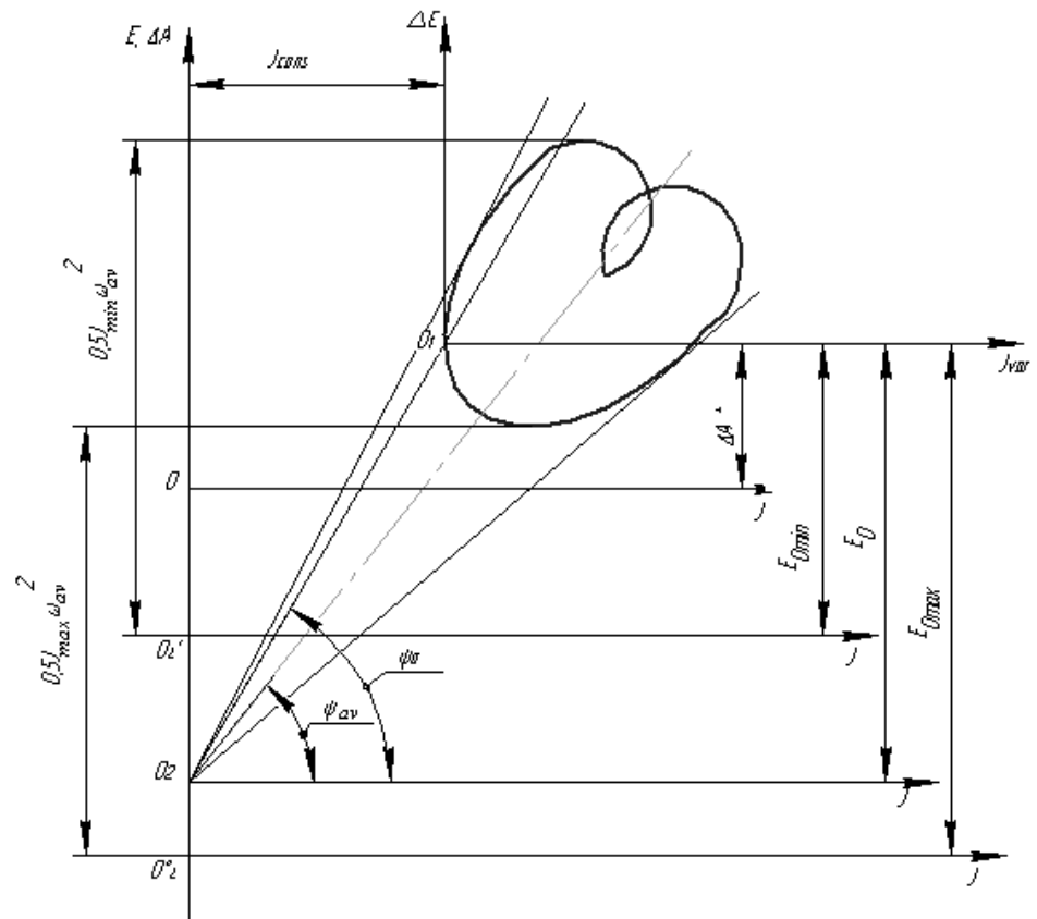
Fig. 1. To the dynamic analysis of the mechanism
