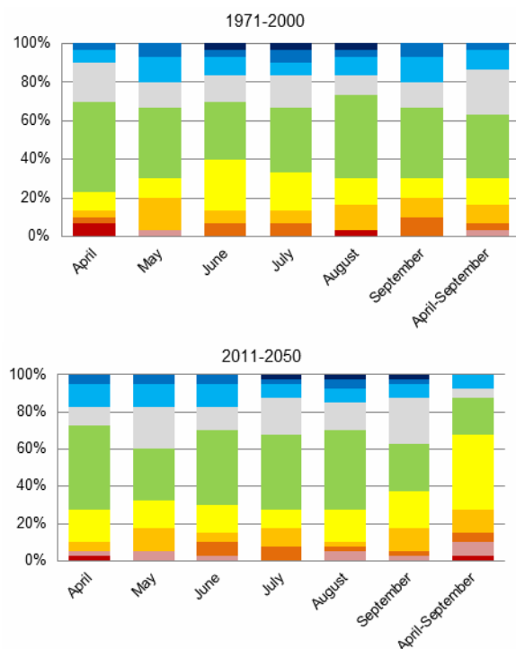
Fig. 2. Frequency of thermal periods in 1971–2000 and 2011–2050; explanations as in Table 4; source: own study
