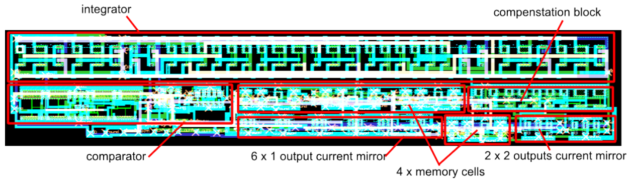
Fig. 7. Sigma-delta modulator layout.
