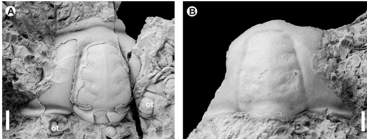
Text-fig. 17. Dunderbergia sp. from the Furongian of Vilske (Vg), Sweden. A – incomplete, partly testaceous cranidium, LO12083t, O. truncatus Zone; B – incomplete cranidium, LO12084t, O. gibbosus or O. truncatus Zone. Accompanying fauna: ot – Olenus truncatus (Brünnich, 1781). Scale bars represent 0.5 cm
