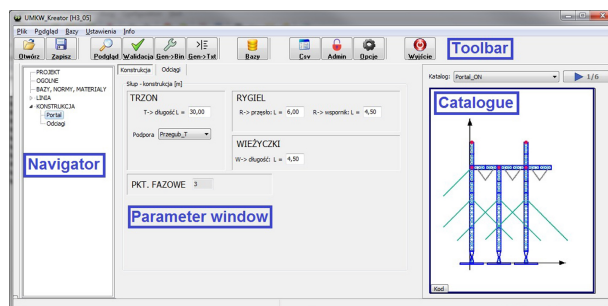
Fig. 5. Interface of the UMKW-Wizard module
