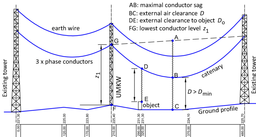
Fig. 8. Determining the elevation of conductor suspension point
