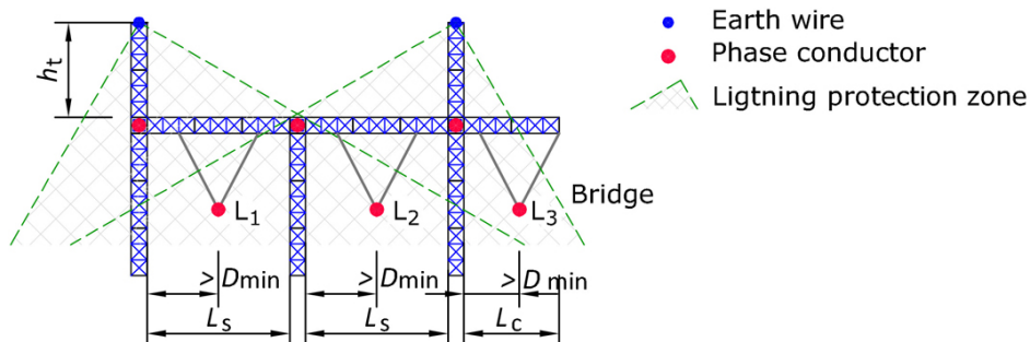
Fig. 7. An angle-tension frame head configuration
