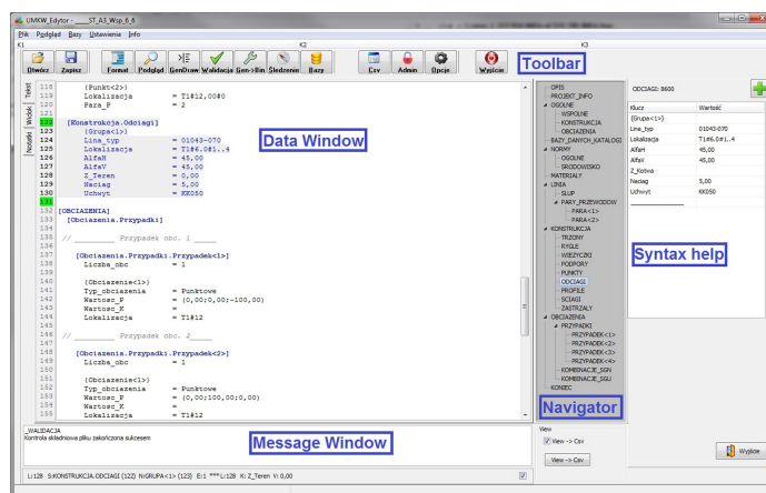
Fig. 6. Interface of the UMKW-Editor module
