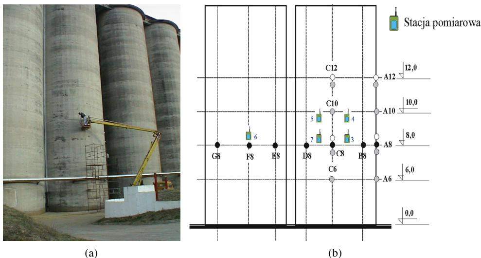
Fig. 2. The battery of cylindrical grain silos: (a) preparation of the silo chambers for testing, (b) diagram of the measurement point layout
