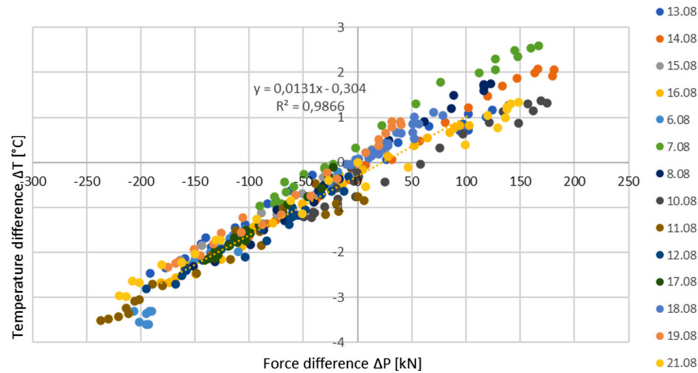
Fig. 11. Dependence of \Delta P on \Delta T in strut 15_2, with trend line and determination coefficient, August 2019
