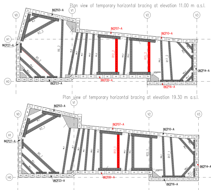
Fig. 1. The plan view of bracing of diaphragm walls in both levels (B1 at elevation 11.00 m and B2 at elevation 19.30 m), locations of inclinometers (INCP) and analyzed steel struts [17]
