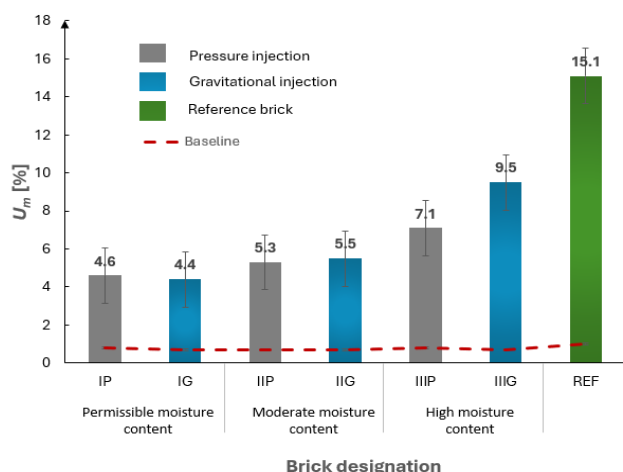
Fig. 8. Average mass moisture values ( U_m ) for re-moistened bricks from groups IP, IG, IIP, IIG, IIIP, IIIG and the reference group (REF)
