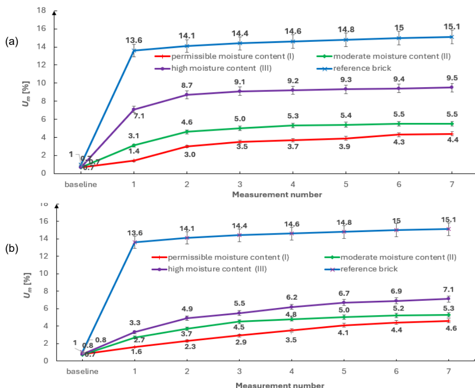
Fig. 11. Comparison of the effectiveness of the protection against moisture with regards to the degree of the moisture content in the bricks at the time of the injection: a) moisture values of the bricks in which gravity injection was performed, b) moisture values of the bricks in which pressure injection was performed
