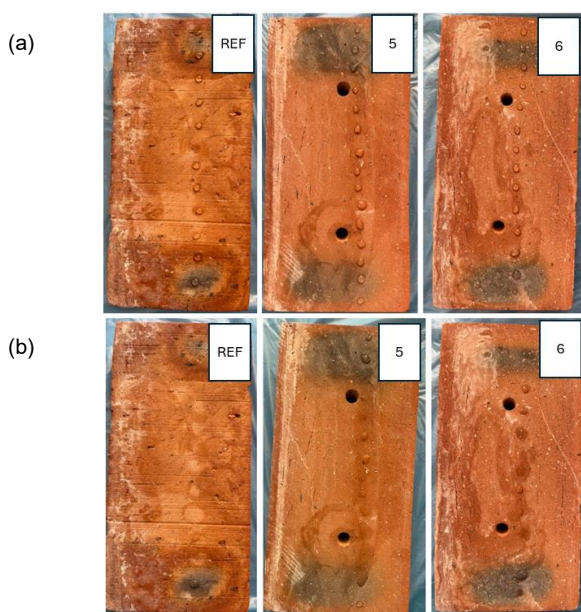
Fig. 12. Water drop tests: a) bricks at the beginning of the test; b) bricks after 2 hours of testing
