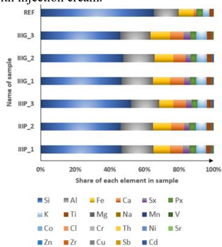
Fig. 15. Percentage share of individual elements in the samples from groups IIIP, IIIG and REF, determined by X-ray fluorescence analysis
