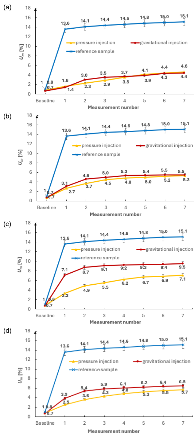
Fig. 10. Comparison of the effectiveness of the protection against moisture in the bricks subjected to pressure and gravity injection, taking into account different degrees of brick moisture content at the time of injection: a) permissible moisture content (IP vs. IG); b) moderate moisture content (IIP vs. IIG); c) high moisture content (IIIP vs. IIIG); d) average values
