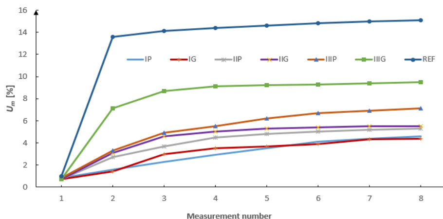
Fig. 9. Changes in the mass moisture content of brick groups IP, IG, IIP, IIG, IIIP, IIIG and REF during the 35-day test
