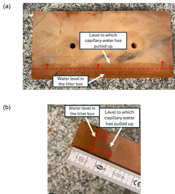
Fig. 6. View of the brick from group IG in the initial phase of water saturation: a) view from the base side; b) view from the head side
