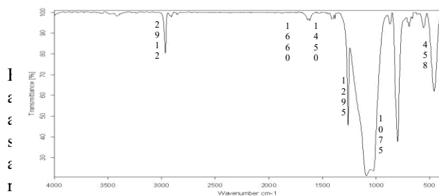
Fig.2. FTIR spectrum of fly ash
