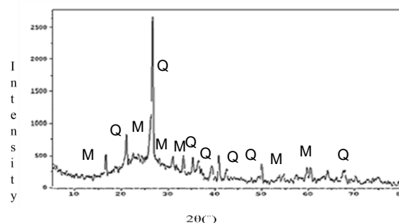
Fig.1. XRD pattern of fly ash
