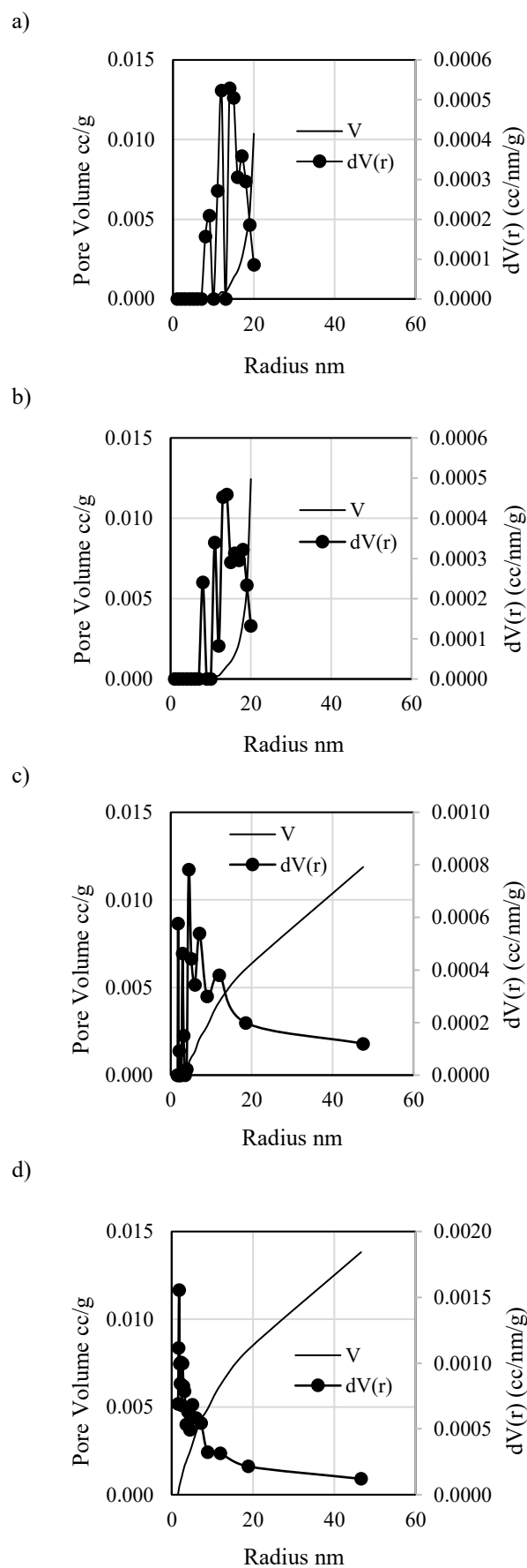
Fig.13. Pore size distribution of the samples of geopolymer foams produced with varying hydrogen peroxide amounts a) 0.5% b) 1% c) 1.5% d) 2%
