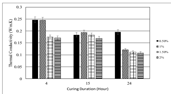
Fig. 4. The thermal conductivity values of geopolymer foams
