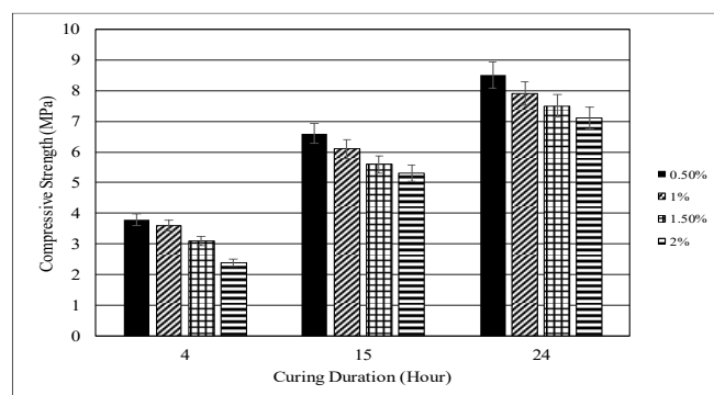
Fig. 5. The compressive strength values of geopolymer foams aged for 7 days
