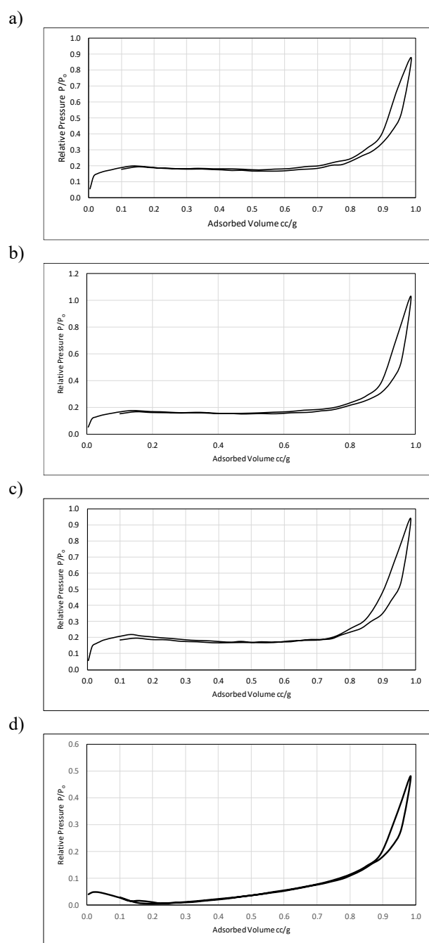
Fig.12. N 2 isotherms of geopolymer foams produced with varying hydrogen peroxide amounts a) 0.5% b) 1% c) 1.5% d) 2%
