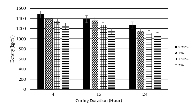
Fig.3. Densities of geopolymer foams
