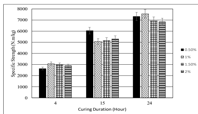
Fig. 7. The specific strengths of geopolymer foams aged for 28 days
