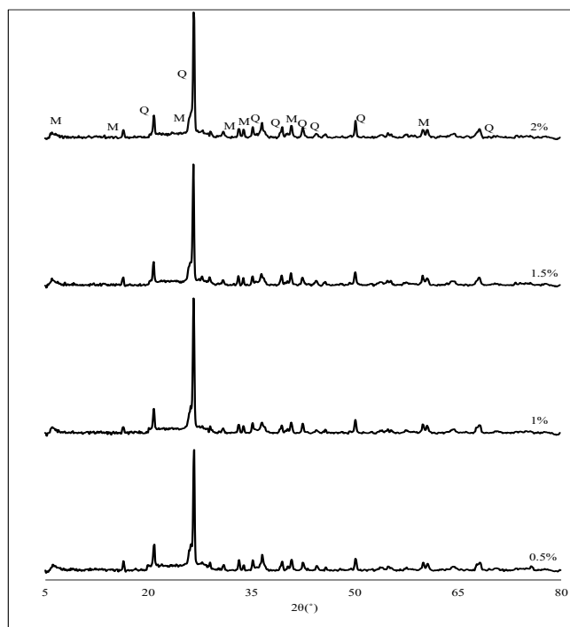
Fig.8. XRD patterns of geopolymer foams
