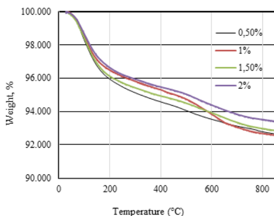
Fig. 11. Thermogravimetric curves of geopolymer foams
