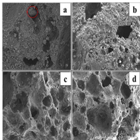
Fig. 10. SEM images of geopolymer foams with x100 magnification a) 0.5% b) 1% c) 1.5% d) 2%
