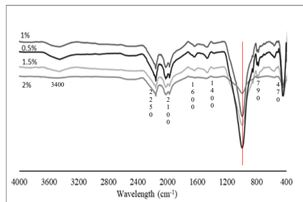
Fig.9. FTIR spectra of geopolymer foams
