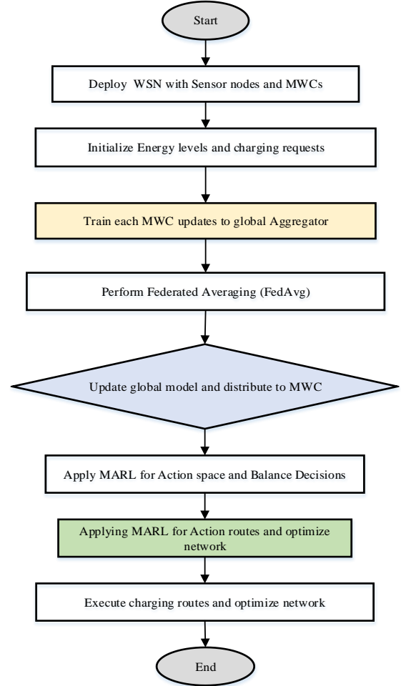
Fig.4. Flowchart for FedRL-MARL execution
