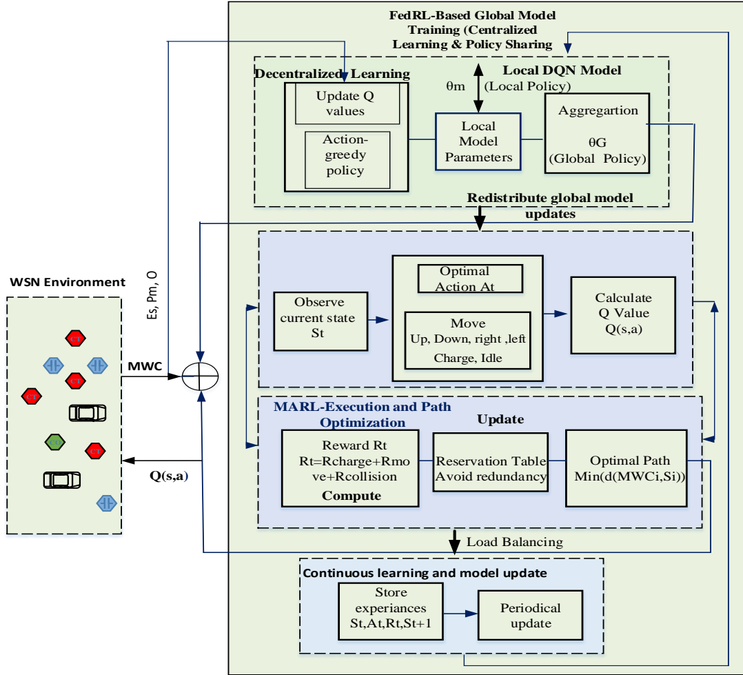
Fig.3. Proposed Architecture of FedRL-MARL Framework
