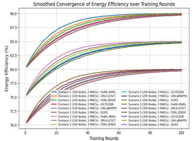
Fig.11. Energy Efficiency Convergence Across Scenarios and Charging Methods
