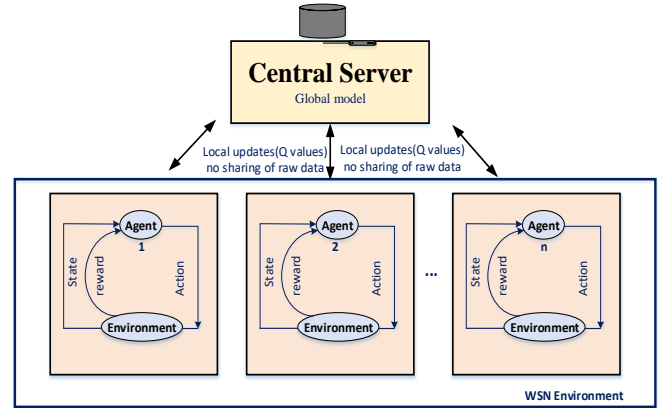
Fig. 2. Federated Learning Framework
