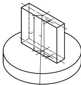
Fig. 2. Central length of the gauge block – l_c [1].
