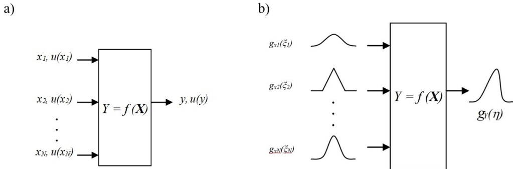
Fig. 3. Difference between the principle of uncertainty evaluation according to: a) the GUM uncertainty framework (GUF), b) the Monte Carlo Method (MCM).
