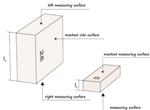
Fig. 1. Gauge blocks and their surfaces.
