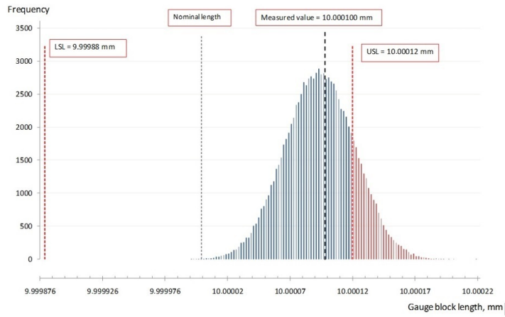
Fig. 8. Assessment of the risk of making a wrong decision using the Monte Carlo uncertainty evaluation (grade 0 gauge blocks).
