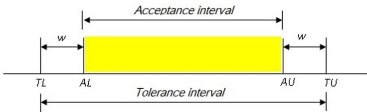
Fig. 4. Guard bands for a two-sided acceptance interval having lower and upper tolerance limits.
