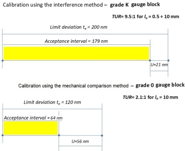
Fig. 7. Guard bands with a width of w = U for calibration by interference and mechanical comparative methods for gauge blocks with the smallest TUR values.
