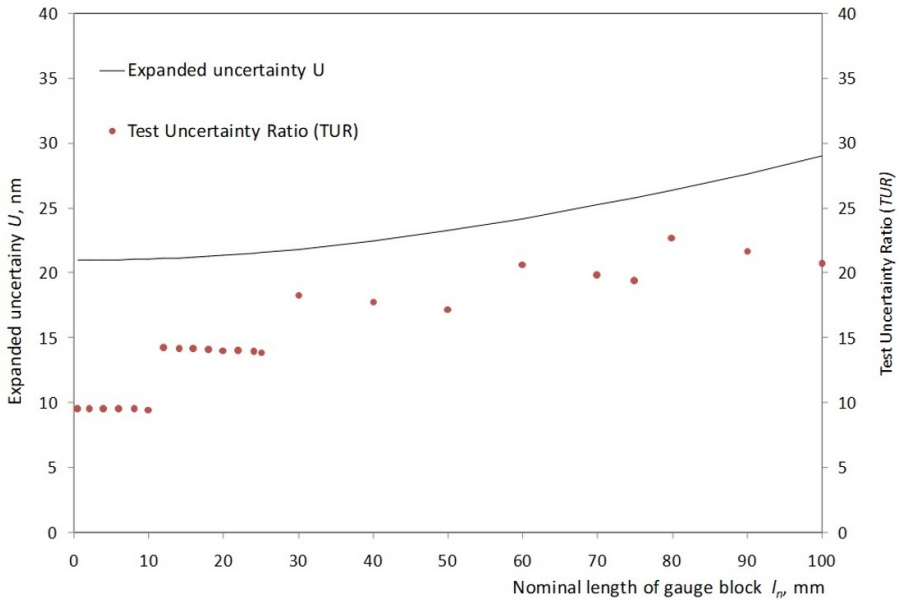
Fig. 5. Test Uncertainty Ratio ( TUR ) for the interferometric calibration method of gauge blocks.
