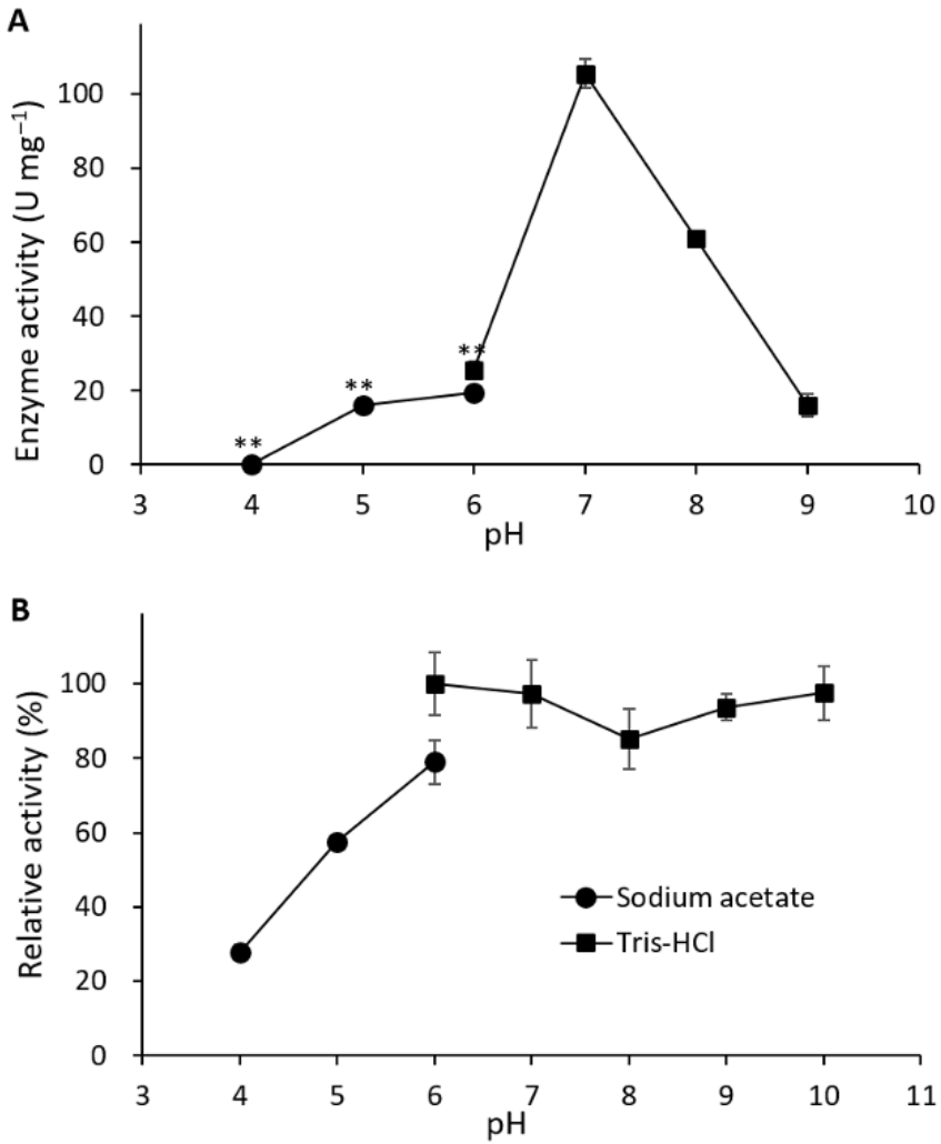
Fig. 4. Effect of pH on amylase activity. (A) Starch-degrading activity (U mg -1 ) of \alpha -amylase from KS7913 at pH 4.0 to 9.0. (B) pH stability of \alpha -amylase from KS7913. To achieve the pH values, the following buffers were used: 50 mM sodium acetate buffer pH 4.0 to 6.0 (●) and 50 mM Tris-HCl buffer pH 6.0 to 10.0 (■). * p < 0.05 and ** p < 0.01 compared to the optimal pH (pH 7.0).
