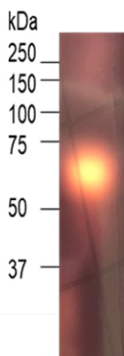
Fig. 3. Activity confirmation of amylase from Alteromonas sp. KS7913 by zymography analysis.
