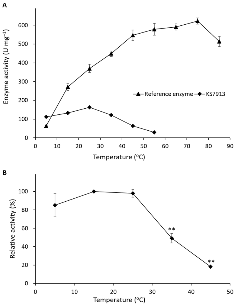
Fig 5. Effect of temperature on amylase activity. (A) Starch-degrading activities ( \text{U mg}^{-1} ) of \alpha -amylase from KS7913 (◆) and the commercially available enzyme (▲) at temperatures ranging from 5°C to 85°C. (B) Thermostability of \alpha -amylase from KS7913. * p < 0.05 and ** p < 0.01 compared to the optimal temperature (25°C).
