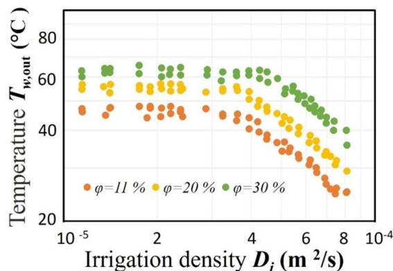
Figure 5: Outlet water temperature versus irrigation density for three different inlet vapour content.
