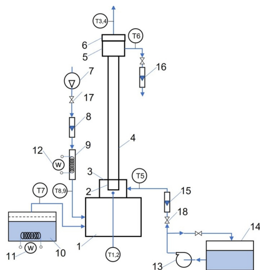
Figure 1: Schematic diagram of experimental installation: 1 – chamber for mixing air and water vapour; 2 – porous insert; 3 – water inlet chamber; 4 – test pipe; 5 – hot water collection chamber; 6 – separator; 7 – compressor; 8, 15, 16 – rotameters; 9 – electric heater; 10 – steam generator; 11, 12 – watt-meters; 13 – pump; 17, 18 – valves; T1-T9 – thermocouples.
