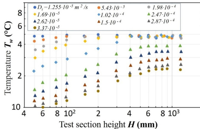
Figure 6: Heating water temperature distribution over the pipe height at initial mixture temperature T_{m,\text{in}} = 105^\circ\text{C} , initial vapour content \varphi = 11\% and mixture velocity W_m = 20.8 \text{ m/s} .
