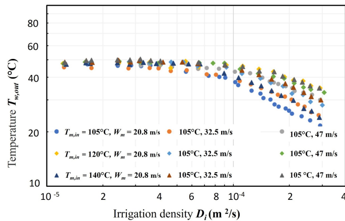
Figure 4: Effect of inlet temperature and velocity of air-vapour mixture on outlet water temperature.
