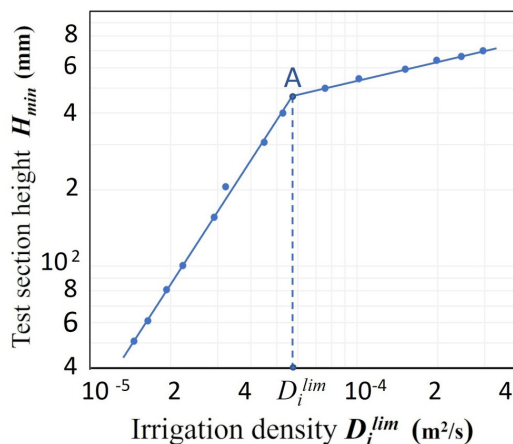
Figure 7: Limiting operating active height of the test section of the pipe versus irrigation density.
