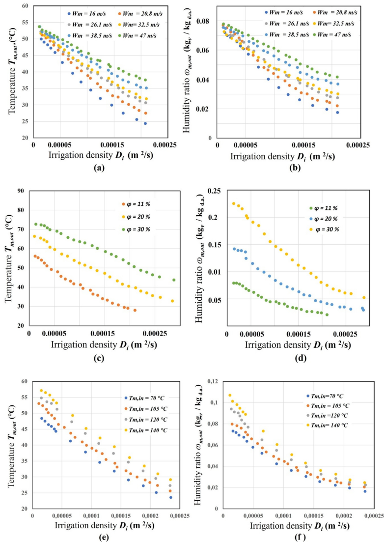
Figure 3: Outlet temperature and humidity ratio of the air-water vapour mixture versus irrigation density for different values: (a), (b) velocity of the AWVM; (c), (d) vapour content of the AWVM; (e), (f) initial temperature of the AWVM.
