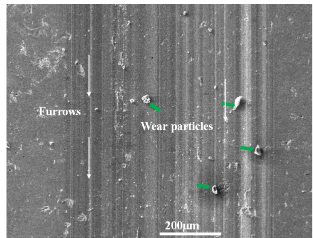
Fig. 11. Surface wear morphology of Ni60/SiO 2 coating surface
