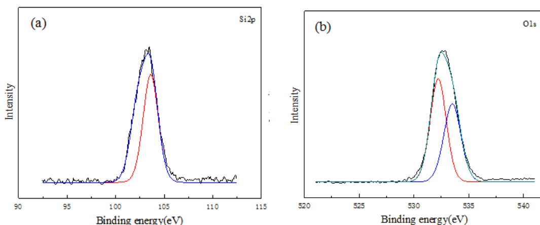
Fig. 4. XPS spectra of rice husk products, (a) Si2p binding energy, (b) O1s binding energy
