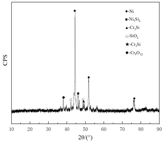
Fig. 8. Phase structure of Ni60/SiO 2 coating
