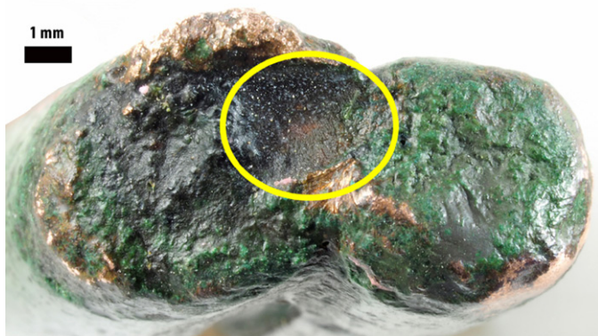
Fig. 23. Location of the defect for the actual necklace casting
