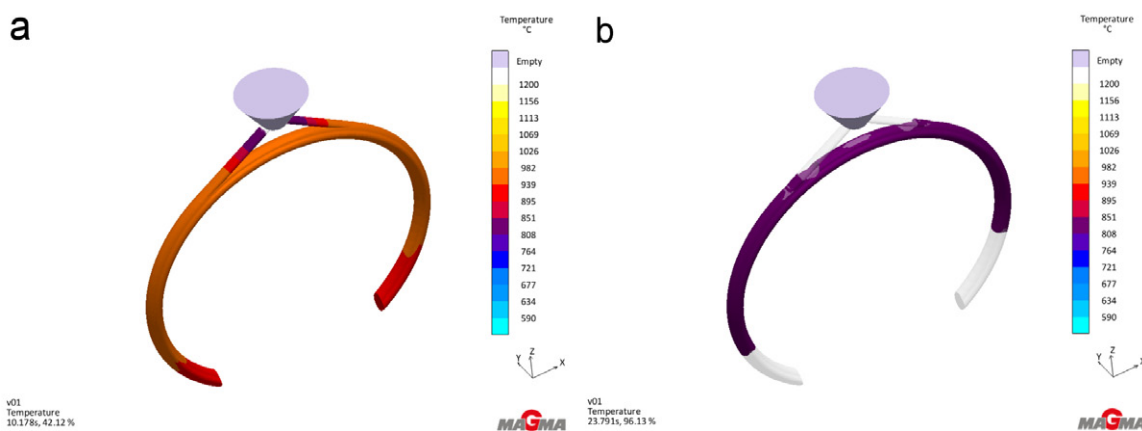
Fig. 21. Temperature distribution during the solidification process: steps 42.12% (a) and 96.13% (b)
