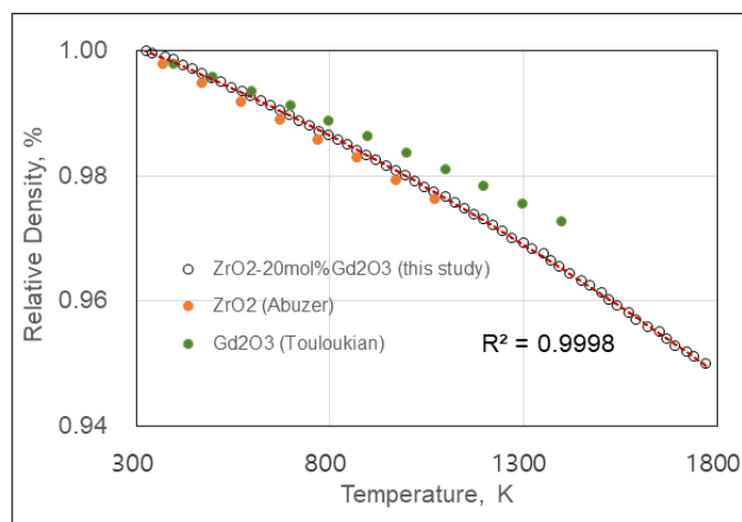
Fig. 5. Relative density of the ZrO_2 -20 mol% Gd_2O_3 pellet as a function of temperature
