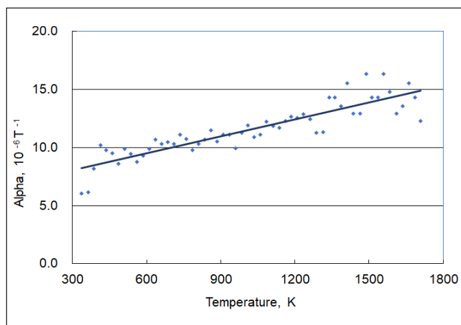
Fig. 4. Instantaneous thermal expansion coefficient of ZrO_2 -20 mol% Gd_2O_3 as a function of temperature
