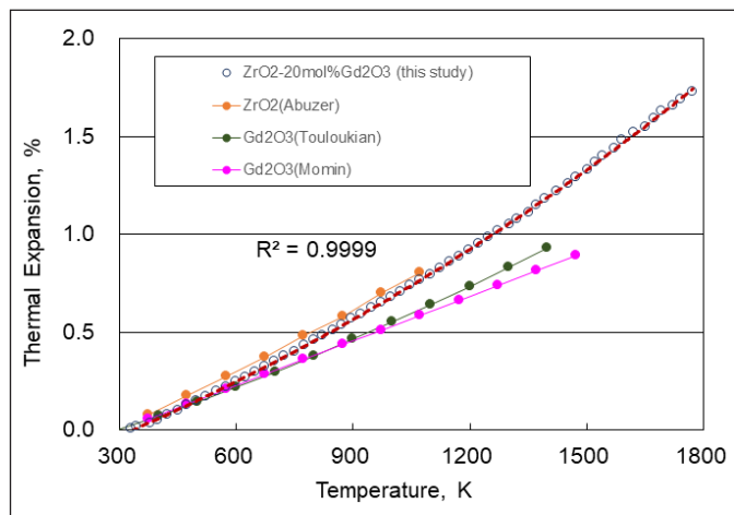
Fig. 3. Linear thermal expansion values of ZrO_2 , Gd_2O_3 , and ZrO_2 -20 mol% Gd_2O_3 as a function of temperature
