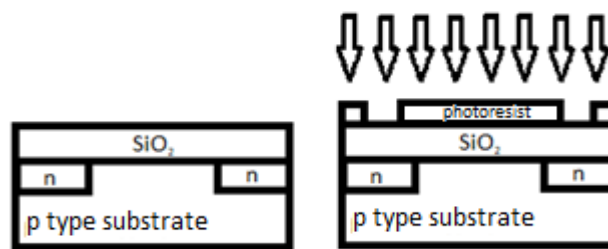
Fig 3. Substrate after deposition of gate oxide (left) and after photolithography enabling the formation of contacts (right)
