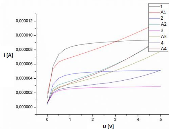
Fig.9. Results of the first stage of the experiment for second transistor
