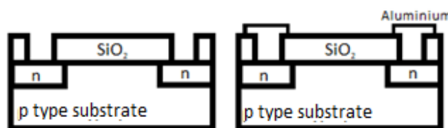
Fig 4. Transistor before making contacts (left) and finished ISFET (right)
