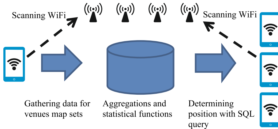
Figure 1 Architecture overview
