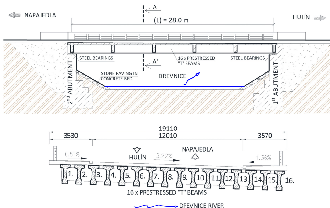
Fig. 2. The longitudinal and cross (A-A') sections of the bridge 551-030
