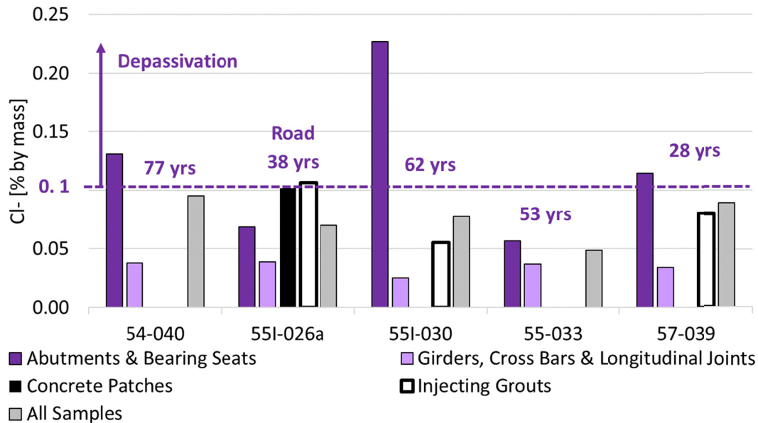
Fig. 5. Water soluble chloride ion concentration Cl^- [wt.-%/cement] [8] for selected bridges and respective construction members
