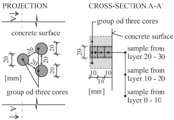
Fig. 1. Illustration of the core samples drilled from one location of the structure
