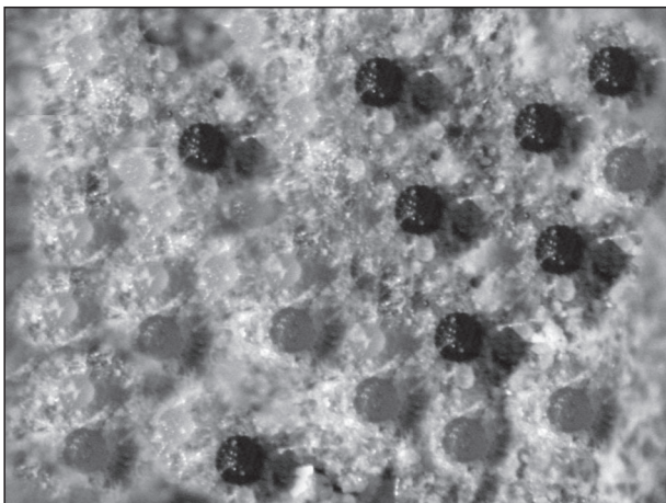
Fig. 8. Cleistothecia of U. necator at different stages of growth on the leaf of a susceptible grape variety
