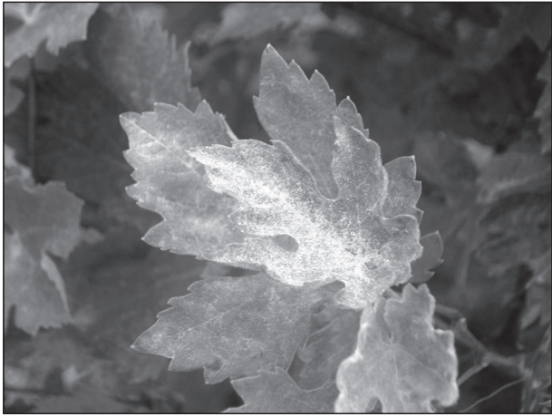
Fig. 1. Severe powdery mildew infection on a susceptible grape variety (Kopakboghan)
