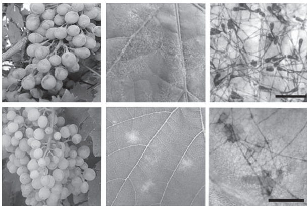
Fig. 7. U. necator -induced symptoms on a susceptible (top) and a resistant (bottom) V. vinifera variety. Left and center panels: appearance of PM-infected leaves and clusters. Right panel: Aniline blue-stained fungal structures as observed under a compound microscope. Note the profuse and sparse fungal growth on the susceptible and resistant genotype, respectively. Scale bar: 100 \mu m
