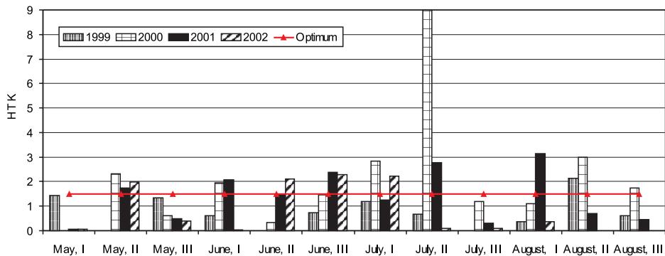
Fig. 1. Hydrothermal coefficient of the flax growing seasons, Uptyt, 1999–2002
