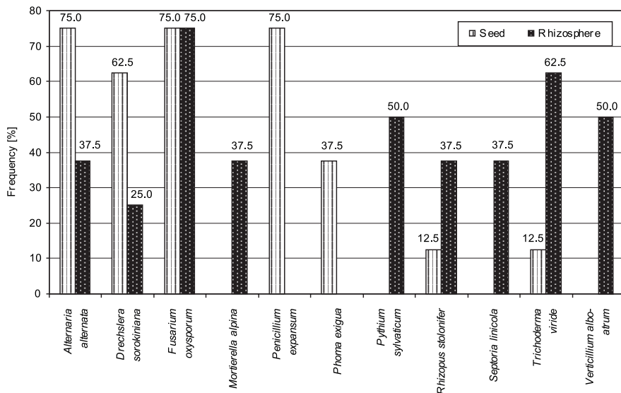
Fig. 2. Frequency of fungal species found on flax seed and in the rhizosphere, Uptyt, 2001
