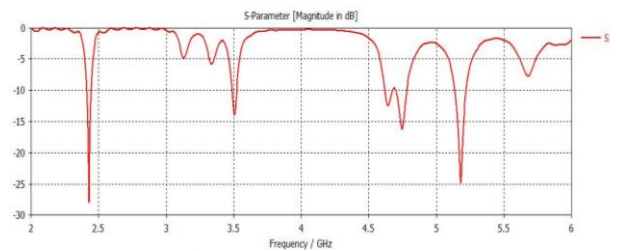
Fig. 3. S_{11} from simulation.
