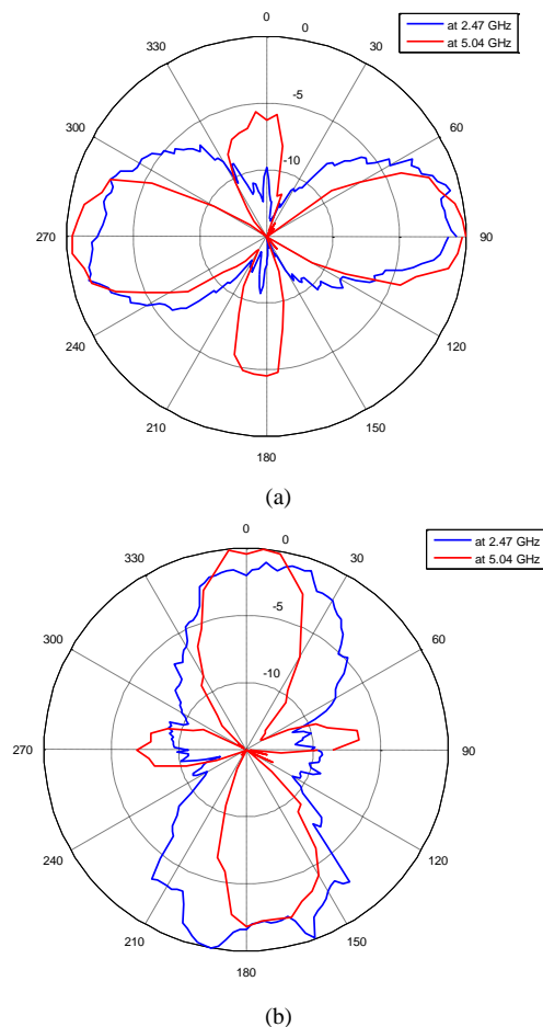
Fig. 7. The radiation patterns from experimental at 2.47 GHz and 5.04 GHz of (a) case A and (b) case B.
