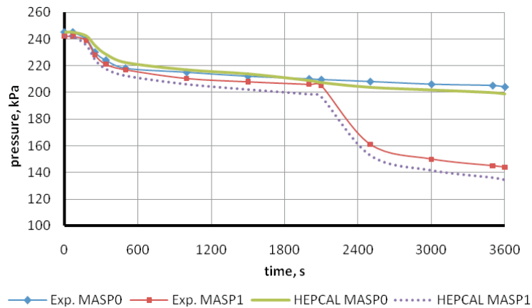
Figure 8. Comparison of pressure trends for the MISTRA test MASPO and MASP1.
