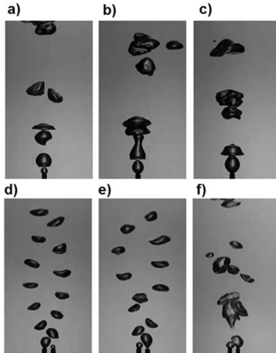
Figure 4. The typical bubble behaviours for bubble chain formation from the single nozzle and two neighbouring nozzles for different air volume flow rates and S = 4 mm: a) single nozzle, q = 0.15 \text{ dm}^3/\text{min} ; b) single nozzle, q = 0.2 \text{ dm}^3/\text{min} ; c) single nozzle, q = 0.3 \text{ dm}^3/\text{min} ; d) two neighbouring nozzles; q = 0.15 \text{ dm}^3/\text{min} ; e) two neighbouring nozzles, q = 0.2 \text{ dm}^3/\text{min} , f) two neighbouring nozzles, q = 0.3 \text{ dm}^3/\text{min} .
