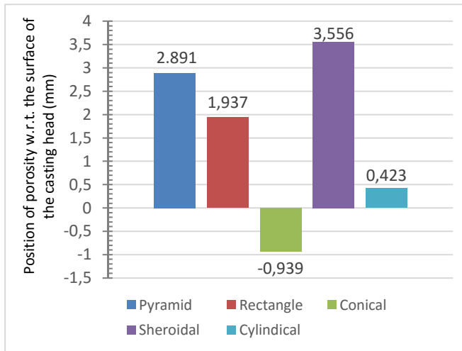
Fig. 15. Position of porosity vs. change of feeder shape
