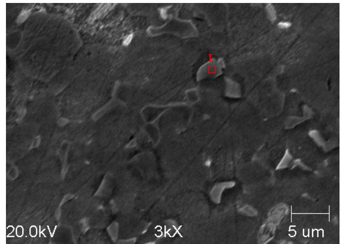
Fig. 4. SEM image representing the microstructure of a two phase titanium alloy, Ti6Al4V at 3000 \times magnification
