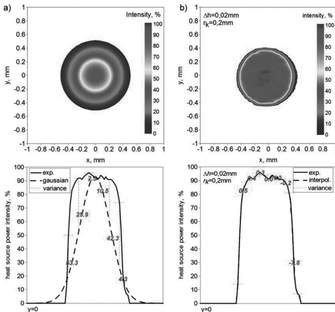
Fig. 7. Percentage distribution of laser power described by a) Gaussian and b) interpolated models
