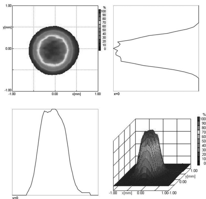
Fig. 3. Experimentally obtained percentage distribution of Yb:YAG laser beam power at beam focusing z=5 mm
