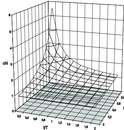
Fig. 1. Function \chi(tT^{-1}, c) from relation (6).
