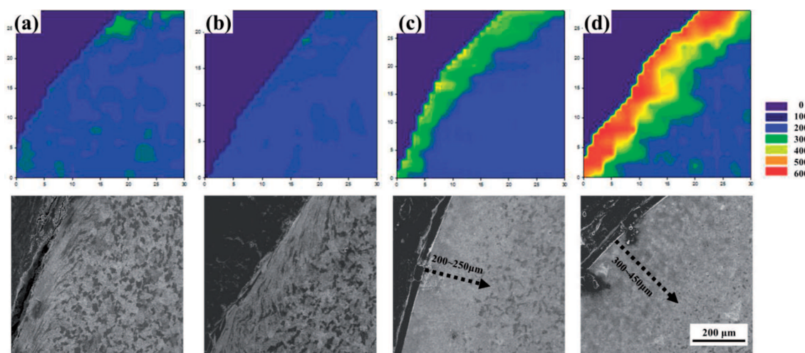
Fig. 4. Distribution of micro-Vickers hardness and corresponding SEM micrographs from the specimens treated by (a) peening-only, (b) 600°C laser heat treatment plus peening, (c) 700°C laser plus peening, and (d) 800°C laser plus peening
