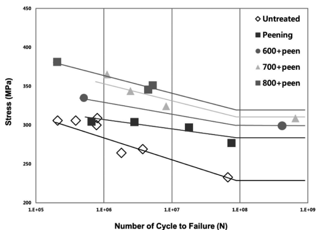
Fig. 2. S-N curves of AISI 4140 from the ultrasonic fatigue test depending on different surface treatment conditions
