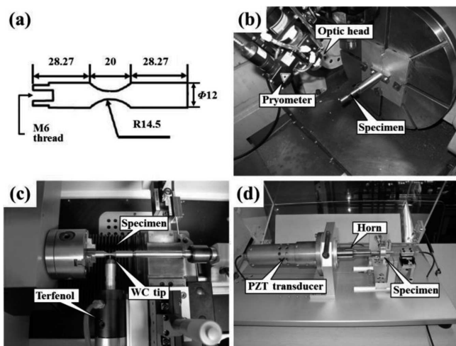
Fig. 1. (a) Fatigue test specimen of AISI 4140, (b) laser heat treatment system, (c) vibration peening system, and (d) ultrasonic fatigue tester
