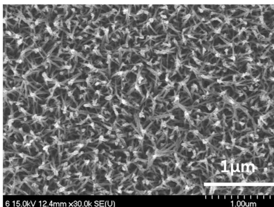
Fig. 1. FE-SEM morphology of the nanorod structures after immersing titanium in 5 M NaOH at 60°C and treating in distilled water at 60°C
