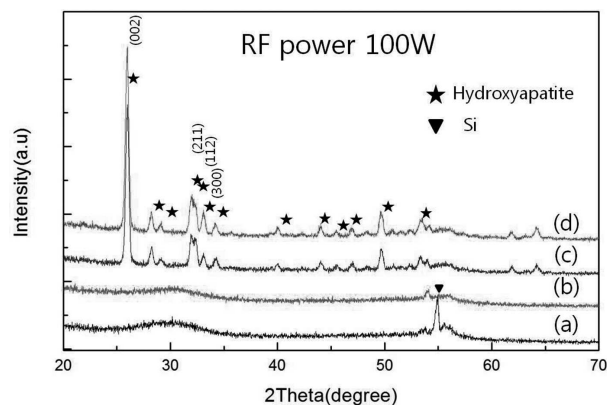
Fig. 2. XRD patterns of the HA thin films coated on an Si substrate after heat treatment: (a) as-sputtered, (b) 400°C, (c) 500°C, and (d) 600°C
