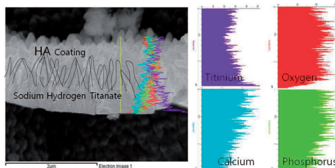
Fig. 5. Cross sectional FE-SEM morphology and EDX line profiles of HA films for a sputtering time of 60 min with heat treatment at 400°C
