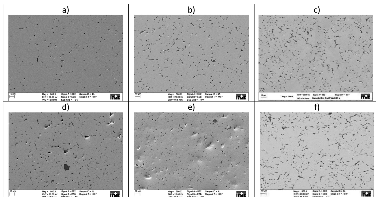
Fig. 5. SEM images of Cu- \text{Al}_2\text{O}_3 composite materials: (a) Cu+1% \text{Al}_2\text{O}_3 HP , (b) Cu+3% \text{Al}_2\text{O}_3 HP , (c) Cu+5% \text{Al}_2\text{O}_3 HP , (d) Cu+1% \text{Al}_2\text{O}_3 TC , (e) Cu+3% \text{Al}_2\text{O}_3 TC , (f) Cu+5% \text{Al}_2\text{O}_3 TC
