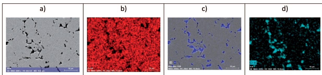
Fig. 6. SEM/EDS maps of the distribution of elements on the surface for Cu+5% \text{Al}_2\text{O}_3 HP (a) SEM image, (b) Cu, (c) Al (d) O
