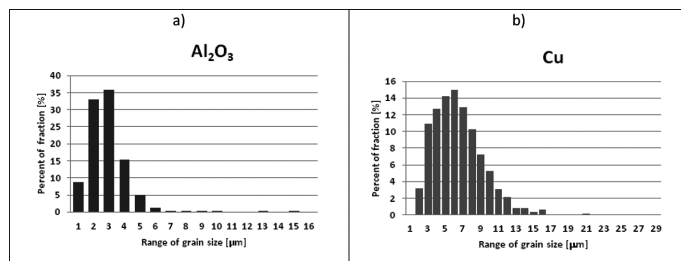
Fig. 1. Distributions of the grain size of (a) Al 2 O 3 and (b) Cu
