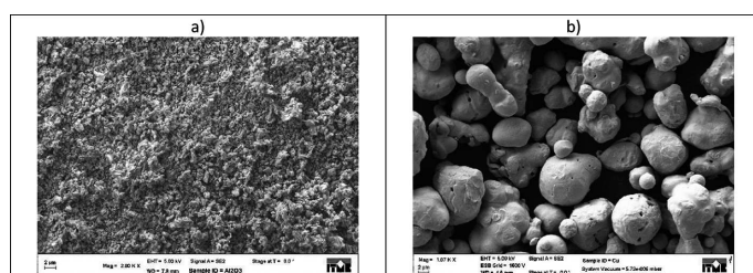
Fig. 2. SEM image of the starting powders (a) Al 2 O 3 and (b) Cu
