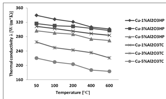
Fig. 8. Thermal conductivity of Cu-Al 2 O 3 composite materials
