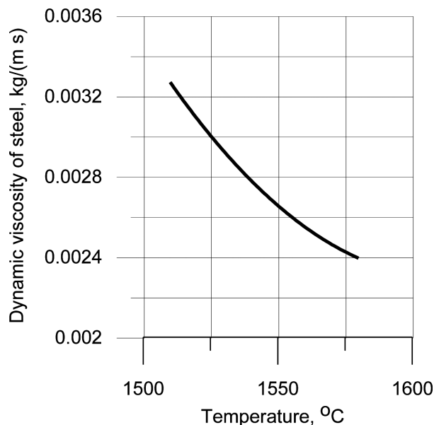
Fig. 3. Liquid steel viscosity [13]
