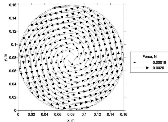
Fig. 8. Force field in the cross section – \varnothing 160 ingot
