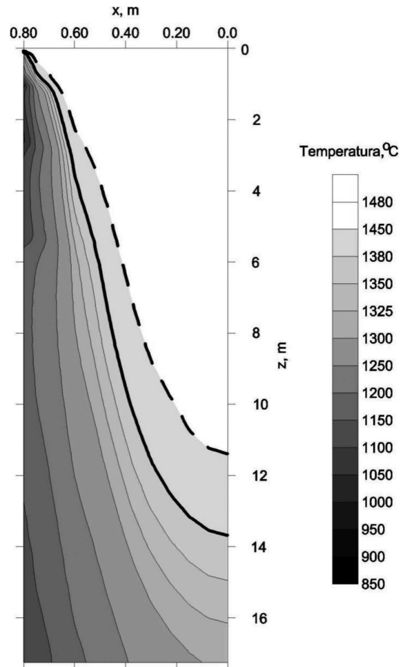
Fig. 6. Temperature field in longitudinal section for \varnothing 160 ingot
