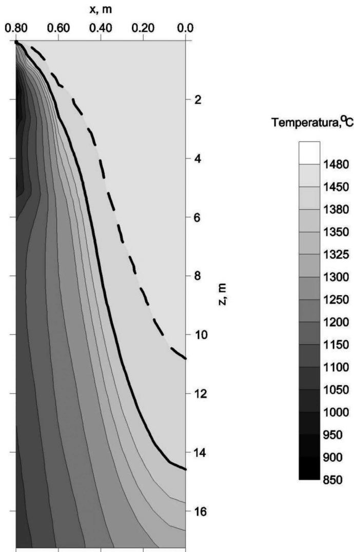
Fig. 5. Temperature field in longitudinal section for 160\times 160 ingot
