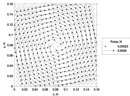
Fig. 7. Force field in the cross section – 160\times 160 ingot
