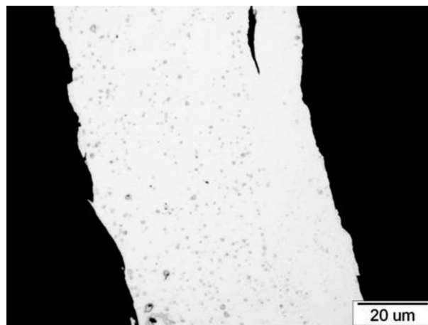
Fig. 9. Microstructure of the AlZn9 alloy flakes
