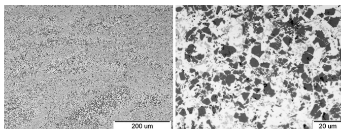
Fig. 10. Microstructure of the AlSi30 alloy rod consolidated by CRE
