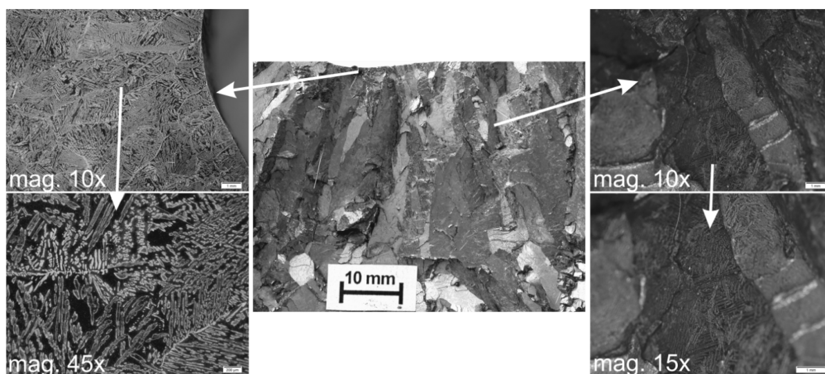
Fig. 1. A fragment of a cracked bulk casting with enlarged columnar crystal zone regions and a primary structure revealed with the Oberhoffer reagent
