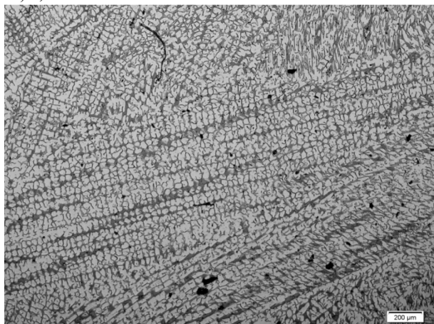
Fig. 2. The microstructure of GX2CrNiMoCuN25-6-3-3 and GX2CrNiMoCuN25-6-3 with varying carbon content
