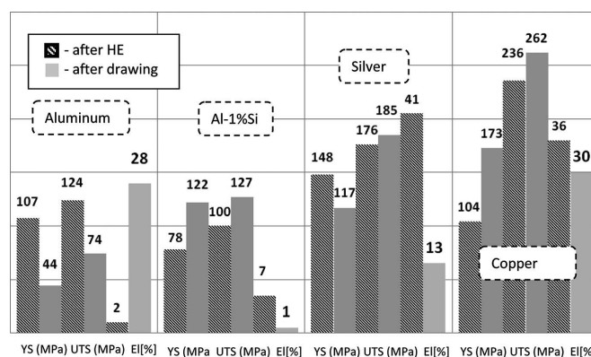
Fig. 7. Yield stress, ultimate tensile strength, and strain to fracture of the HE-processed aluminum, silicon-aluminum alloy, silver, and copper wires compared with the properties of drawn commercial wires
