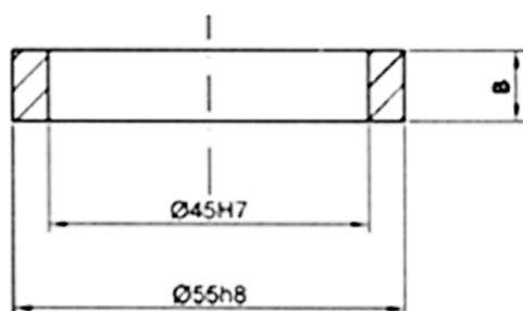
Fig. 2. The design of sample used for the measurement of weight loss during tests carried out on an apparatus available at the Institute of Mining Mechanisation: B – the sample width: upper B = 10 mm, bottom B = 6 mm
