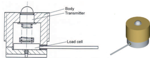
Fig. 13. Compactability sensor
