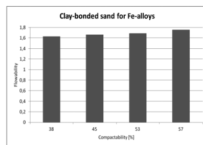
Fig. 23. Compactability-flowability-diagramm of clay-bonded praxis sand for Fe-alloys
