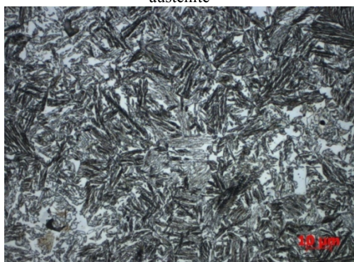
Fig. 8. Microstructure of ADI from C5 cycle. Etched with Beraha reagent - Martensite, 1000x. Pre-eutectoid ferrite, lower bainite, austenite
