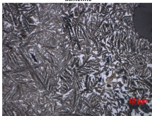
Fig. 9. Microstructure of ADI from C6 cycle. Etched with Beraha reagent - Martensite, 1000x. Pre-eutectoid ferrite, lower bainite, austenite
