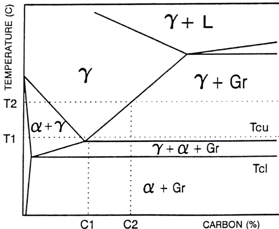
Fig. 1. Qualitative 2 D image of the phase equilibrium diagram for a ternary Fe-C-Si system containing 2,5% Si. \gamma – austenite, \alpha – ferrite, G – grahite, Tcu –upper critical austenitising temperature, Tcl –lower critical austenitising temperature [4]
