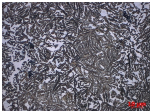
Fig. 7. Microstructure of ADI from C4 cycle. Etched with Beraha reagent - Martensite, 1000x. Pre-eutectoid ferrite, lower bainite, austenite
