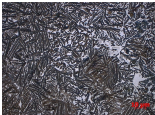
Fig. 4. Microstructure of ADI from C1 cycle. Etched with Beraha reagent - Martensite, 1000x. Pre-eutectoid ferrite, lower bainite, austenite
