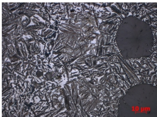
Fig. 6. Microstructure of ADI from C3 cycle. Etched with Beraha reagent - Martensite, 1000x. Pre-eutectoid ferrite, lower bainite, austenite
