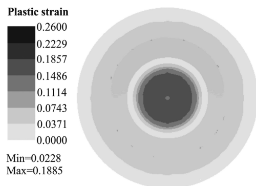
Fig. 6. Plastic strain distribution in the drawn-part made of Gr 2 sheet for the diversified frictional conditions: "punch – blank" \mu = 0.3 , "die – blank" and "blank – blank-holder" \mu = 0.1 , and holding-down force of 1.5 kN
