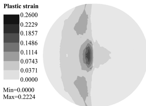
Fig. 10. Plastic strain distribution in the drawn-part made of the welded blank Gr 2 || Gr 5 for the following frictional conditions: “punch – blank” \mu = 0.3 , “die – blank” and “blank – blank-holder” \mu = 0.1 , holding-down force at the onset of crack is 1.5 kN
