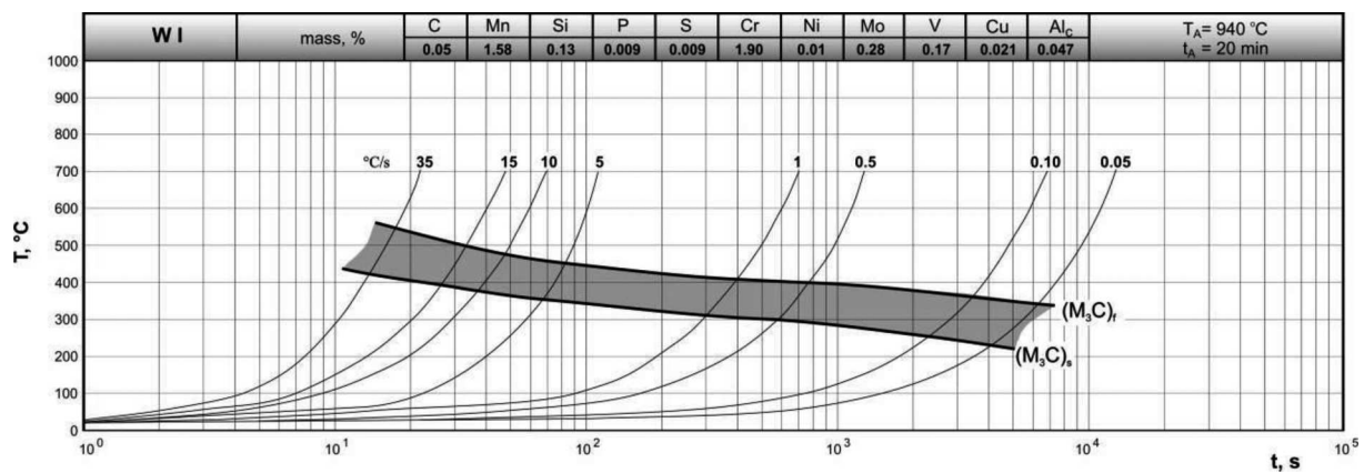
Fig. 5. The CHT diagram of W I steel
