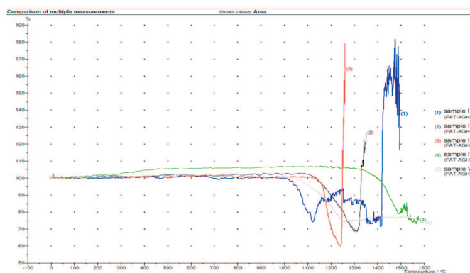
Fig. 6. Changes in the surface areas of samples in the function of temperature
