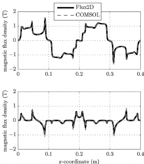
Fig. 5. Comparison of calculated air gap magnetic flux density using transient magnetic simulation with H-formulation in COMSOL and static magnetic simulation in Flux2D. Top: x-component of the air gap magnetic flux density. Bottom: y-component of the air gap magnetic flux density
