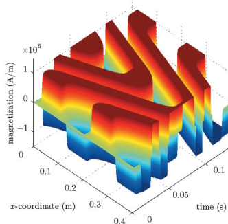
Fig. 3. Magnetization of the magnet region, as function of time and x -coordinate
