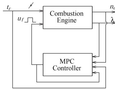
Figure 5. Control scheme
