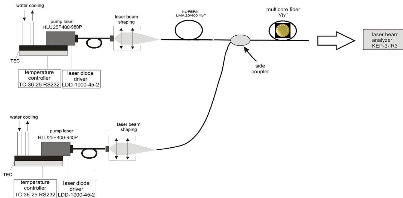
Fig. 12. Experimental setup
