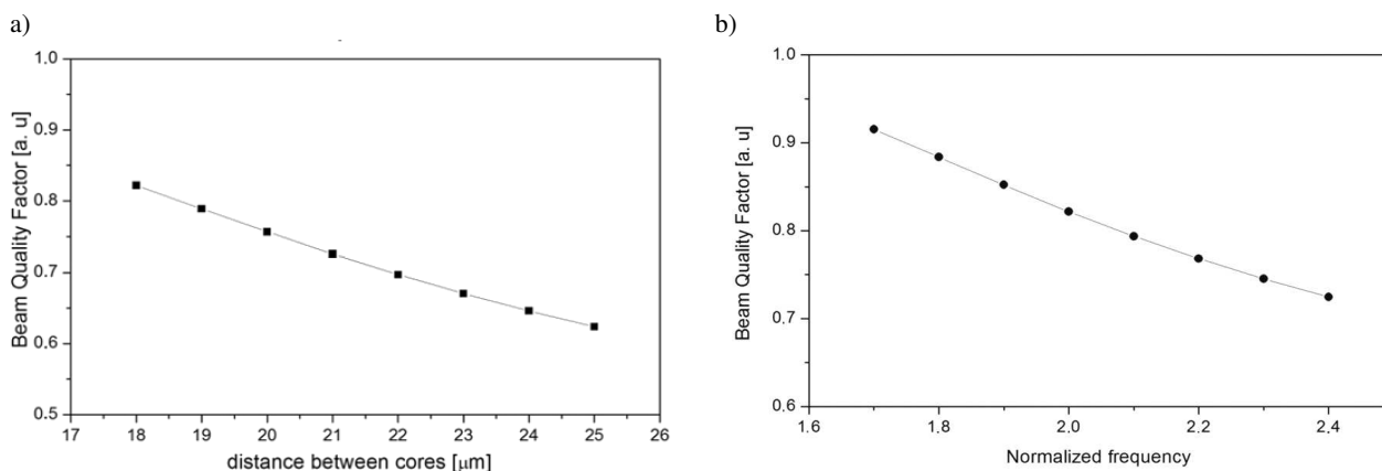
Fig. 6. Relation between BQF and: distance between cores (a), normalized frequency value (b) in the 19-core fibre
