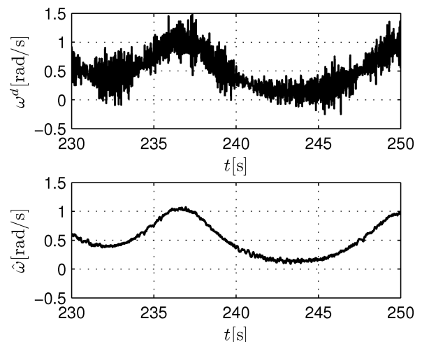
Fig. 8. Estimated velocity \omega by difference estimator ( \omega^d ) and EKF ( \hat{\omega} )
