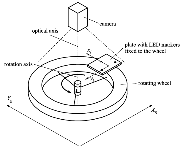
Fig. 5. Experimental setup for static and dynamic accuracy evaluation
