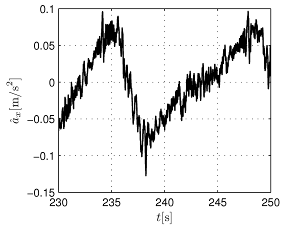
Fig. 10. Estimated accelerations
