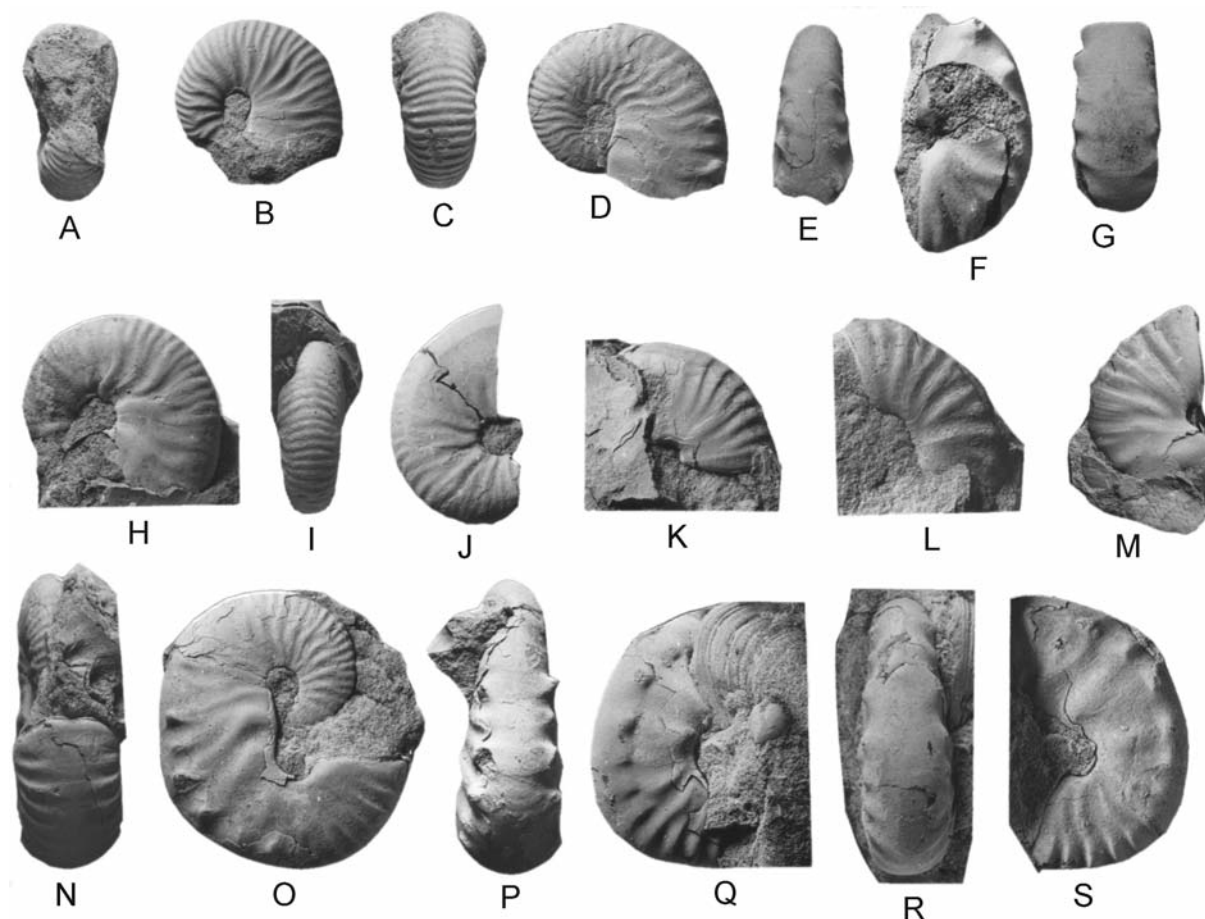
Text-fig. 7. A-S – Yezoites australis sp. nov. A-C – OUM KX5041; D, E – OUM KX7813; F, G – OUM KX7814; H, I – OUM KX5049; J – OUM KX5033; K – OUM KX5042b; L – OUM KX5036; M – OUM KX5035; A-K, M – are paratypes, from bed B of the Upper Santonian St Lucia Formation at locality 105, cliff section on the northern end of the southern peninsula in Lake St Lucia, 3.5 km north of the mouth of the Nyalazi River, ESE of Hluhluwe, 28° 03' 27" S 32° 23' 08" E. N-P, SAM-PCZ22271, probably from locality 105. Q-S – OUM KX7811, a paratype from the Upper Santonian part of the Mzamba Formation at locality 1, cliff and foreshore exposures 1 km north of the mouth of the Mzamba River, Eastern Cape Province, coordinates 31° 05' 50" S, 30° 10' 30" E. All figures are ×1.5.
