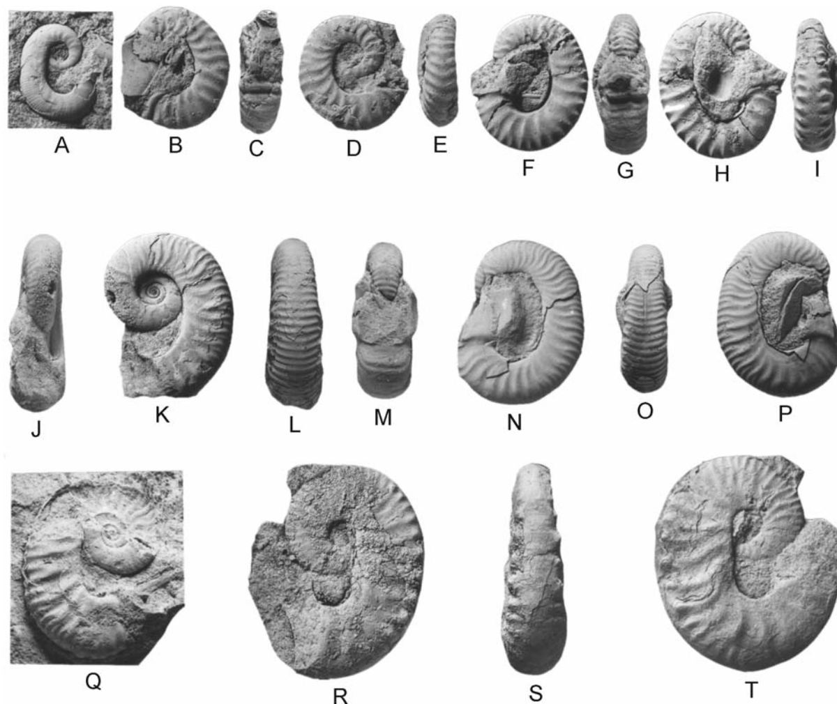
Text-fig. 5. A – Yezoites sp., SAM-PCZ 22245, from the St Lucia Formation at locality 10 of Kennedy and Klinger (1975, p. 282), railroad cutting on the eastern flank of Umkwelane Hill, south of Mtubatuba in northern KwaZulu-Natal, 28° 27' 49" S 32° 09' 58" E. The specimen is probably of Coniacian date. B–I – Argentoscaphites corrugatus sp. nov. B–E – paratype SAM-PCZ 22275, F–I – the holotype, SAM-PCZ 22274, both from the Santonian to Lower Campanian Mzamba Formation at locality 1 of Kennedy and Klinger (1975 p. 281; see also Klinger and Kennedy 1980a): cliff and foreshore exposures 1 km north of the mouth of the Mzamba River, Eastern Cape Province, coordinates 31° 05' 50" S, 30° 10' 30" E. J–T, Yezoites concinna sp. nov. J–L – the holotype, SAM-PCZ22269, from west of locality 93 of Kennedy and Klinger (1975, p. 295), hill slopes ESE of Hluhluwe, 28° 03' 19" S, 32° 20' 00" E. M–P – paratype OUM KX17220; Q – paratype OUM KX17224, both from locality 13 of Kennedy and Klinger (1975, p. 283): Hill slopes below Riverview Compound, 750 m north of the cane railway bridge across the Mfolozi, south of Mtubatuba, 28° 26' 52" S, 32° 10' 48" E. R–T – paratype OUM KX17226, from locality 14 of Kennedy and Klinger (1975, p. 283), road cuttings below the compound immediately south of the Msunduzi River, 2.1 km NNE of Mfolozi, south of Mtubatuba, 28° 28' 24" S 32° 10' 43" E. All specimens are from the Middle Coniacian part of the St Lucia Formation. All figures are \times 1.5 .
