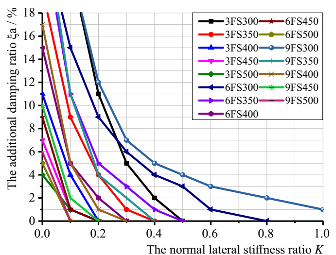
Fig. 8. Group III relationship graphs of the normal lateral stiffness ratio and additional damping ratio
