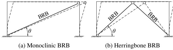
Fig. 2. Schematic diagram of two types of BRB
