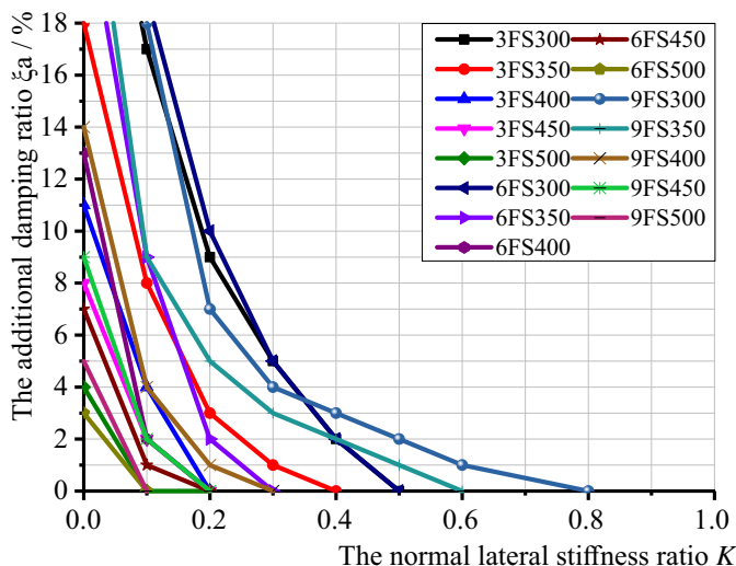
Fig. 9. Group III relationship graphs of the normal lateral stiffness ratio and additional damping ratio
