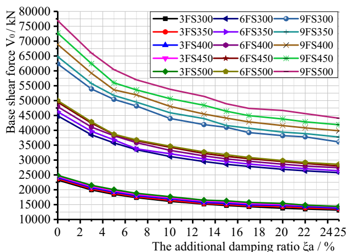
Fig. 7. Group III relationship graphs of the additional damping ratio and base shear force
