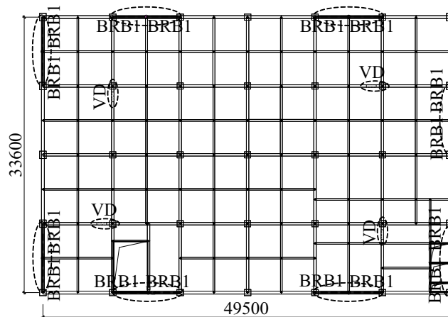
Fig. 10. Layout of dampers
