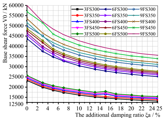
Fig. 6. Group II relationship graphs of the additional damping ratio and base shear force
