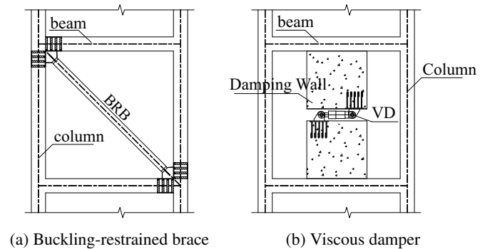
Fig. 1. Schematic diagram of a damper
