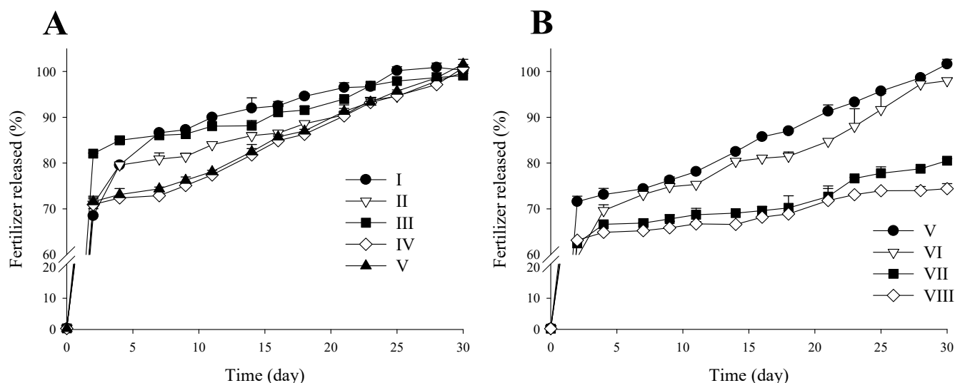
Fig. 1. Influence of the HPMC/EC ratios (A) and PSD ratios (B) on the fertilizer release from controlled-release fertilizer extrusion granules
