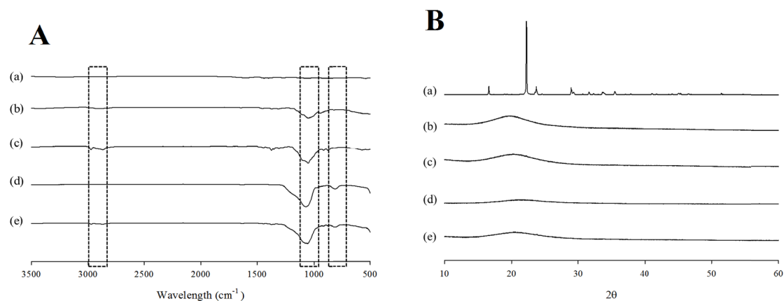
Fig. 3. FT-IR spectra (A) and XRD patterns (B) of Fertilizer (a), HPMC (b), EC (c), PSD (d), and PSD-based controlled-release fertilizer extrusion granules (formulation VII) (e)
