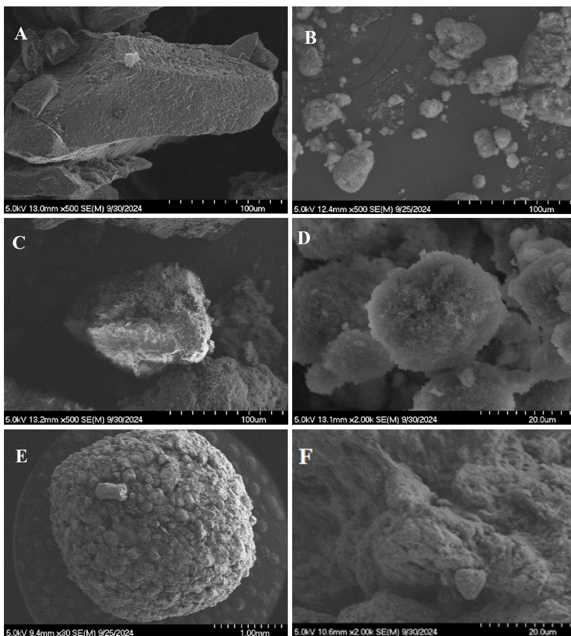
Fig. 2. SEM images of Fertilizer ( \times 500 ) (A), HPMC ( \times 500 ) (B), EC ( \times 500 ) (C), PSD ( \times 2,000 ) (D), PSD-based controlled-release fertilizer extrusion granules (formulation VII, \times 30 ) (E), and PSD-based controlled-release fertilizer extrusion granules (formulation VII, \times 2,000 ) (F)
