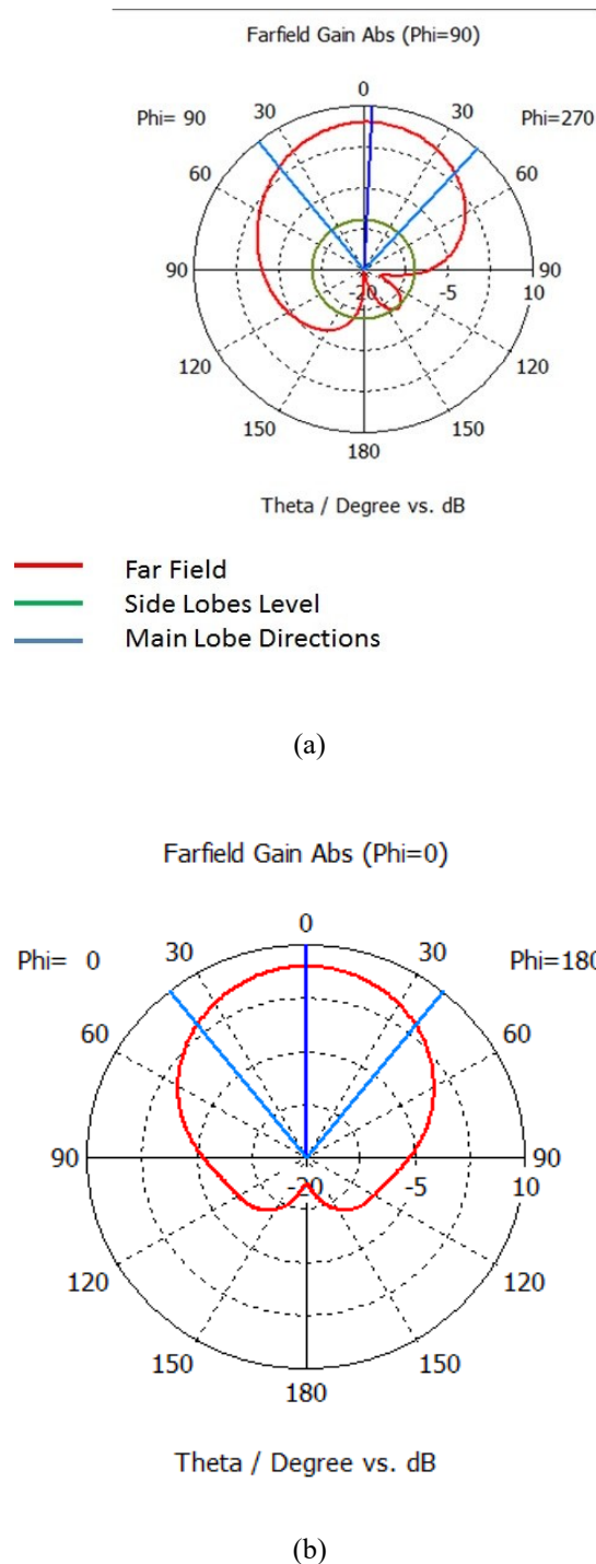
Fig. 4. Far Field For The Proposed Antenna Design: (a) \Phi = 90 and (b) \Phi = 0 Degrees
