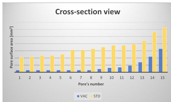
Fig. 9. Pore area – data from block cross-section
