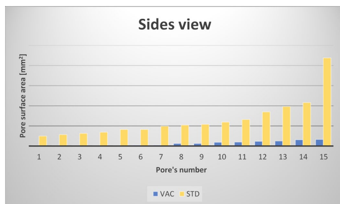
Fig. 8. Pore area – data from the side of the block
