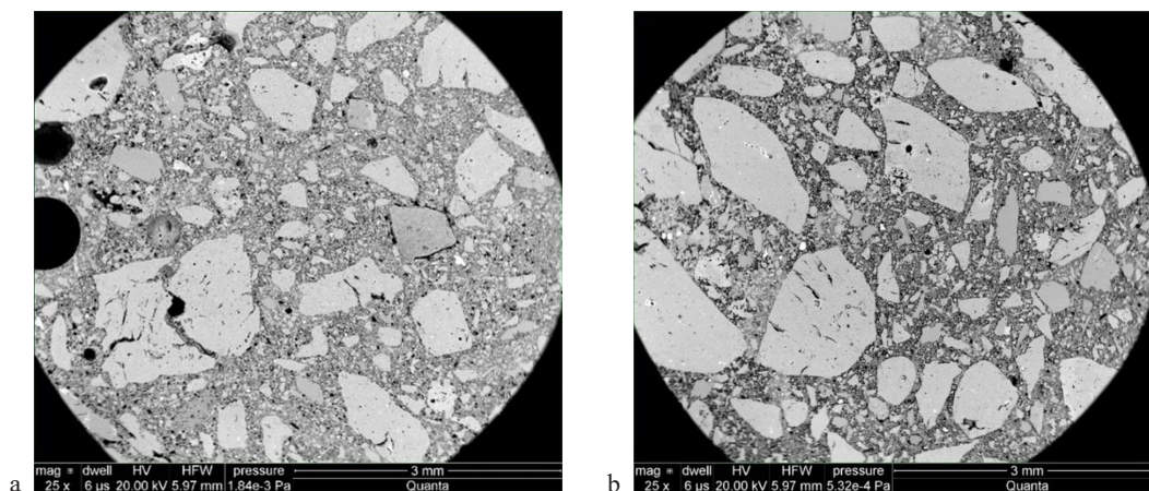
Fig. 13. Photograph of the sample structure at \times 25 magnification; a – STD1, b – VAC1
