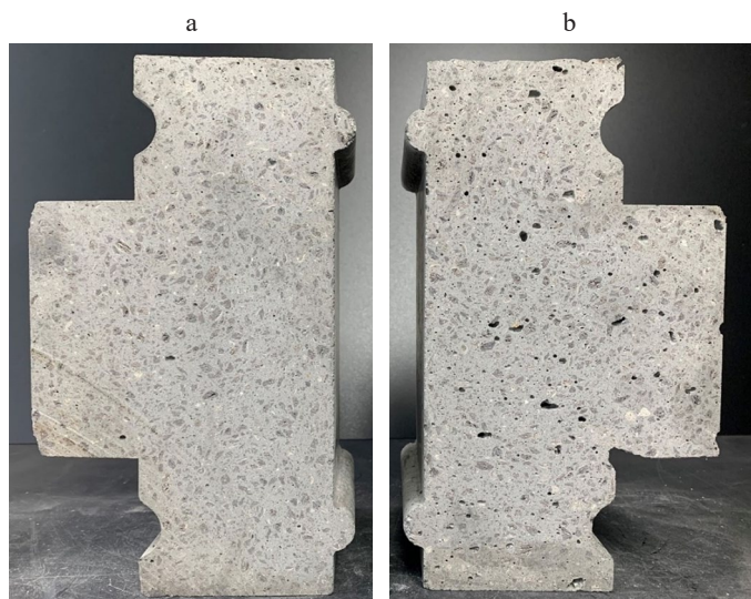
Fig. 5. Comparison of cross-sectional areas of blocks; a – VAC, b – STD
