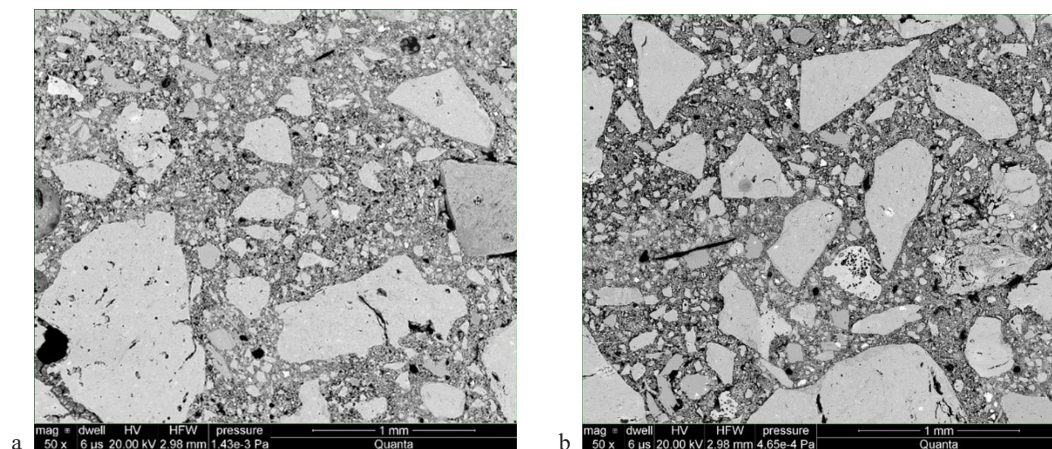
Fig. 14. Photograph of the sample structure at \times 50 magnification; a – STD1, b – VAC1
