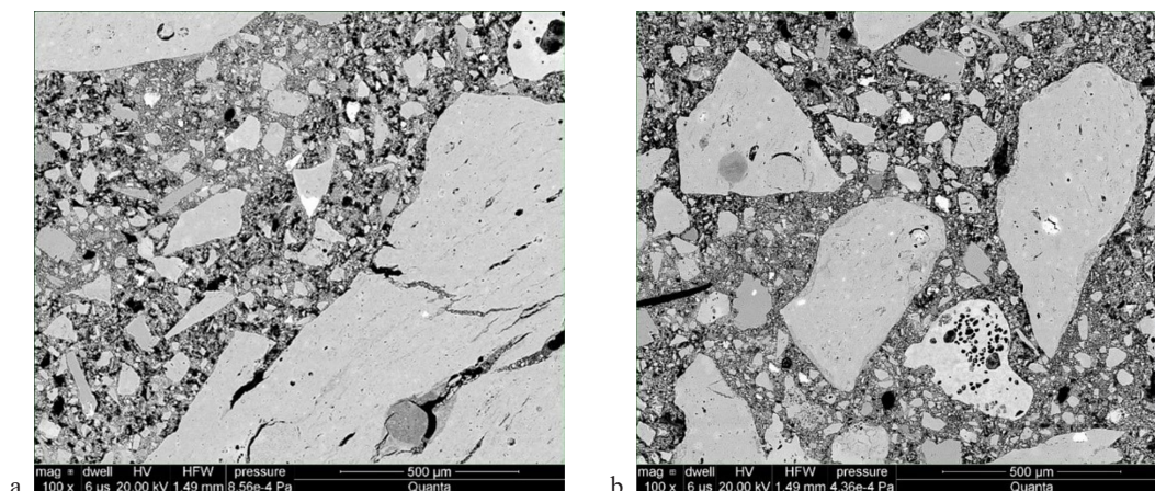
Fig. 15. Photograph of the sample structure at \times 100 magnification; a – STD1, b – VAC1
